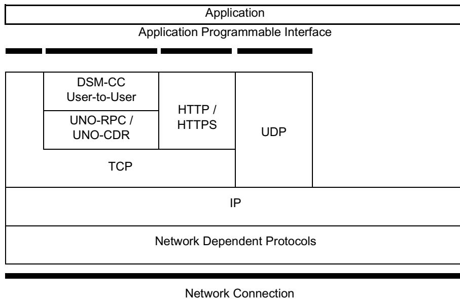
Figure 10: Interaction Channel Protocol Stack
