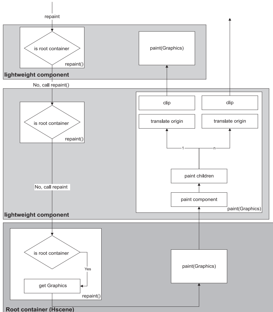
Figure 31: Repaint model in the MHP
