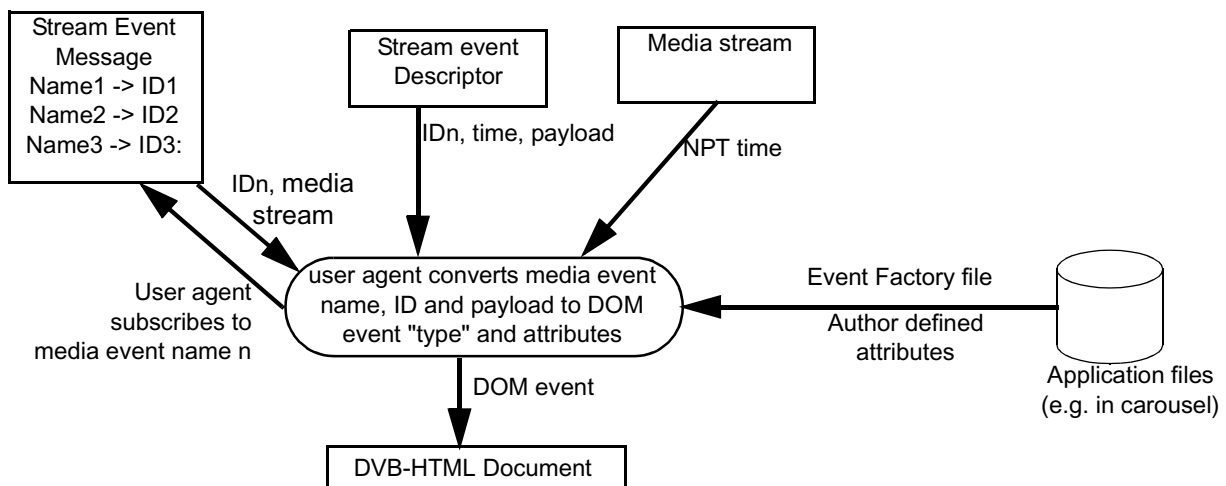
Figure 12: Overview of the authored event mechanism
