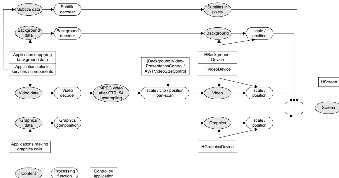
Figure 28: Graphics, Video and Subtitle pipeline
