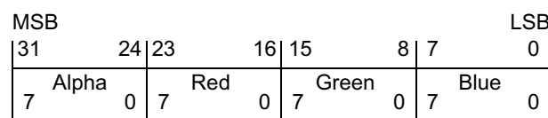
Figure 35: MHP colour format ( TYPE_INT_ARGB )
