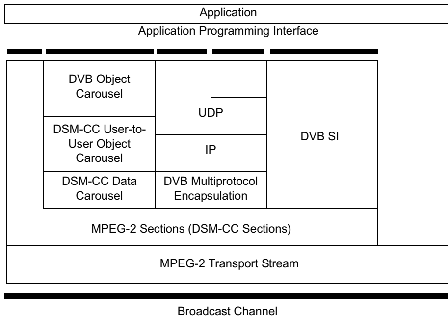
Figure 9: Broadcast Channel Protocol Stack
