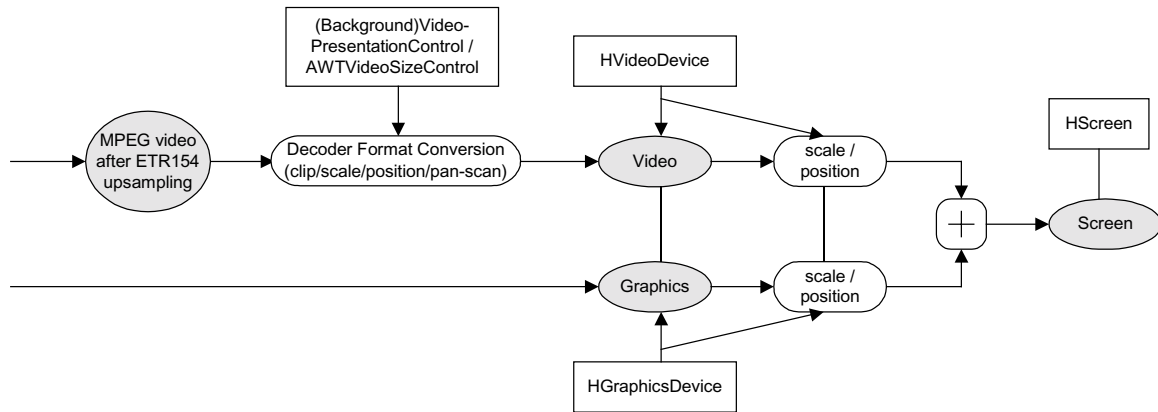
Figure 32: Video and graphics pixel impact
