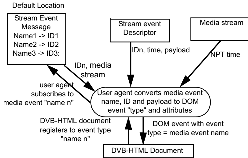
Figure 13: Overview of the default trigger mechanism
