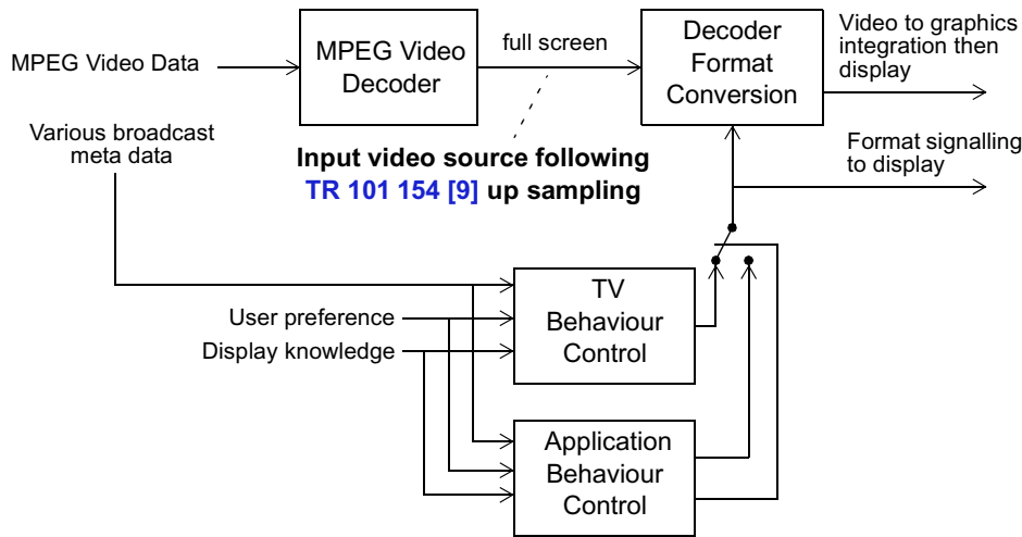
Figure 37: Format control in the presence of a JMF player
