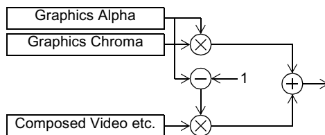
Figure 41: Typical current technology implementation
