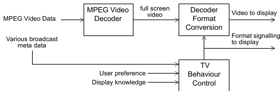
Figure 36: Format control in TV mode
