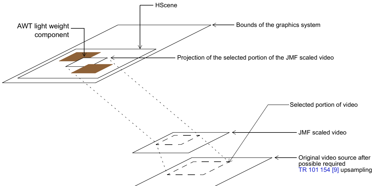
Figure 39: Introducing video into the AWT component stack
